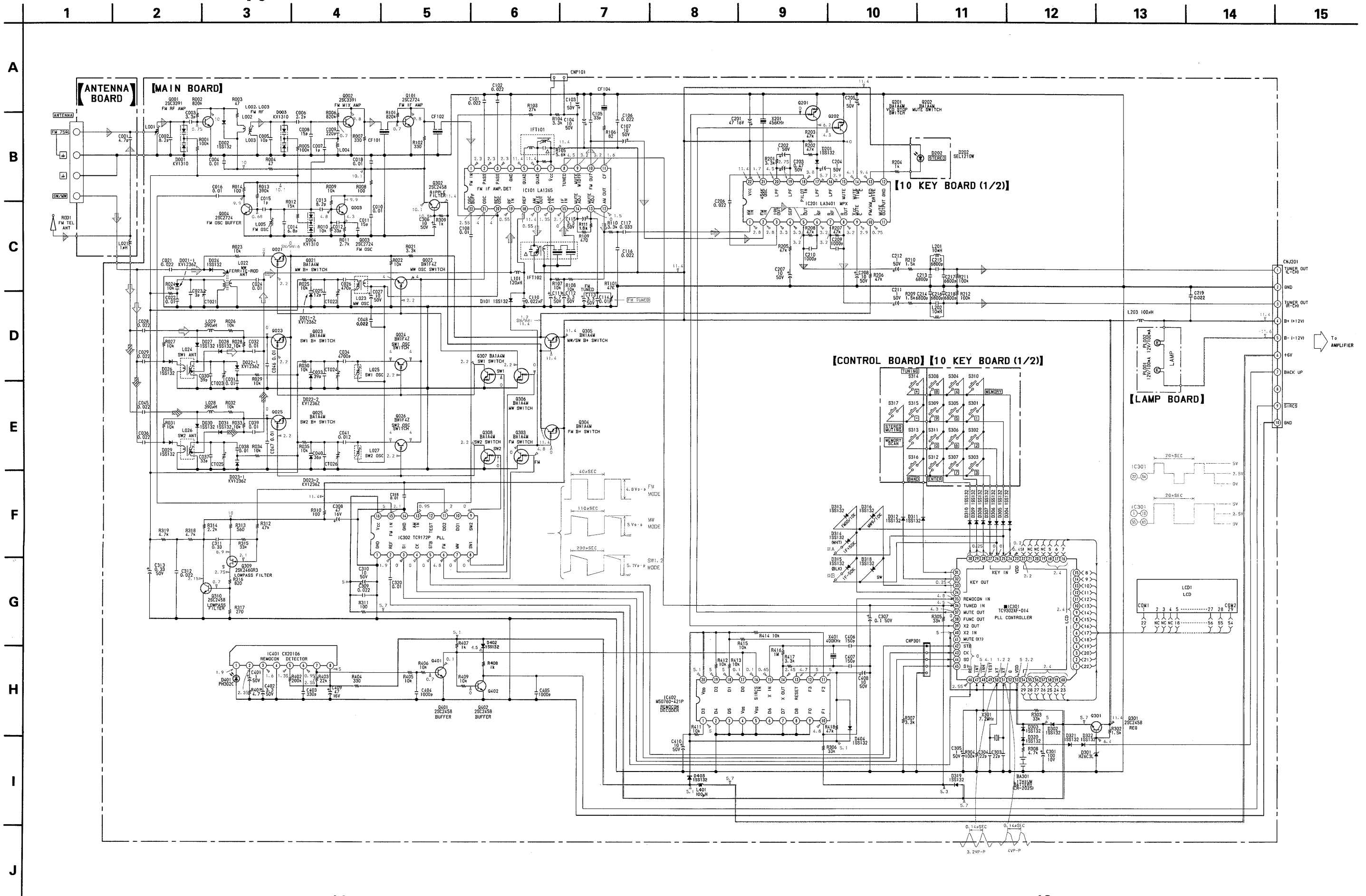
2-2. SCHEMATIC DIAGRAM . See page 13 for note.
